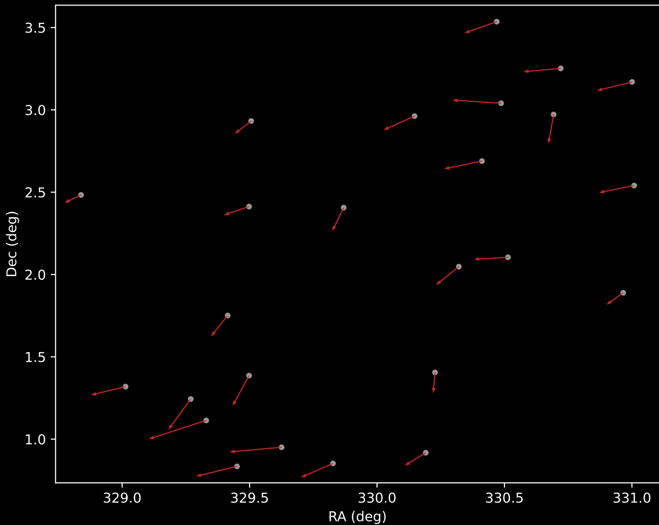
APOGEE DR17 Cluster 6 Proper Motion Vectors (n=25)
