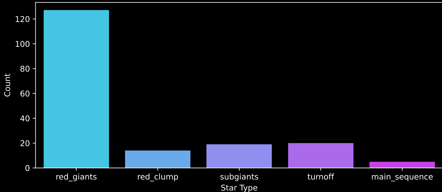
APOGEE DR17 Field: [M5] Count plot of Star Type
