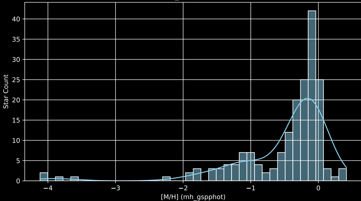
APOGEE DR17 Field: [M5 [M/H] (mh_gspphot) (n= 185)
