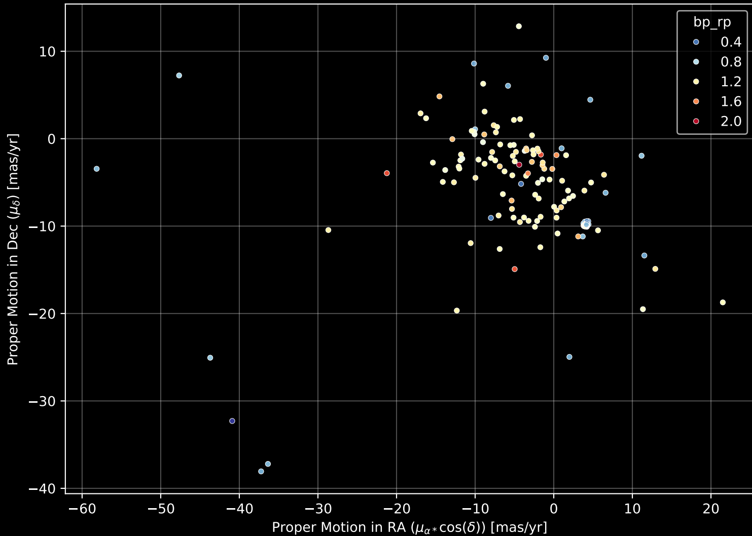
APOGEE DR17 Field: [M5] Proper Motion Diagram (n= 185)
