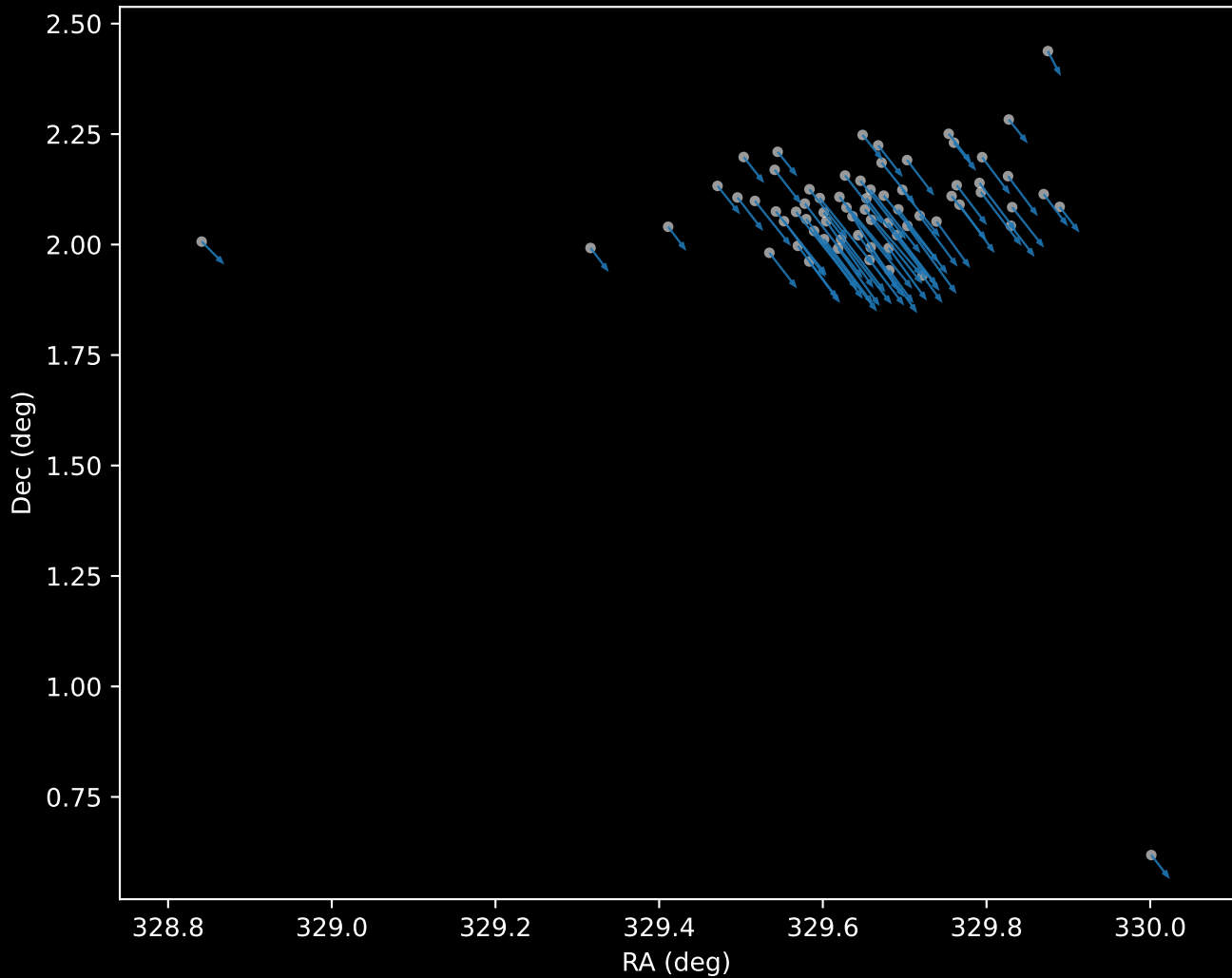
APOGEE DR17 Cluster 0 Proper Motion Vectors (n=68)
