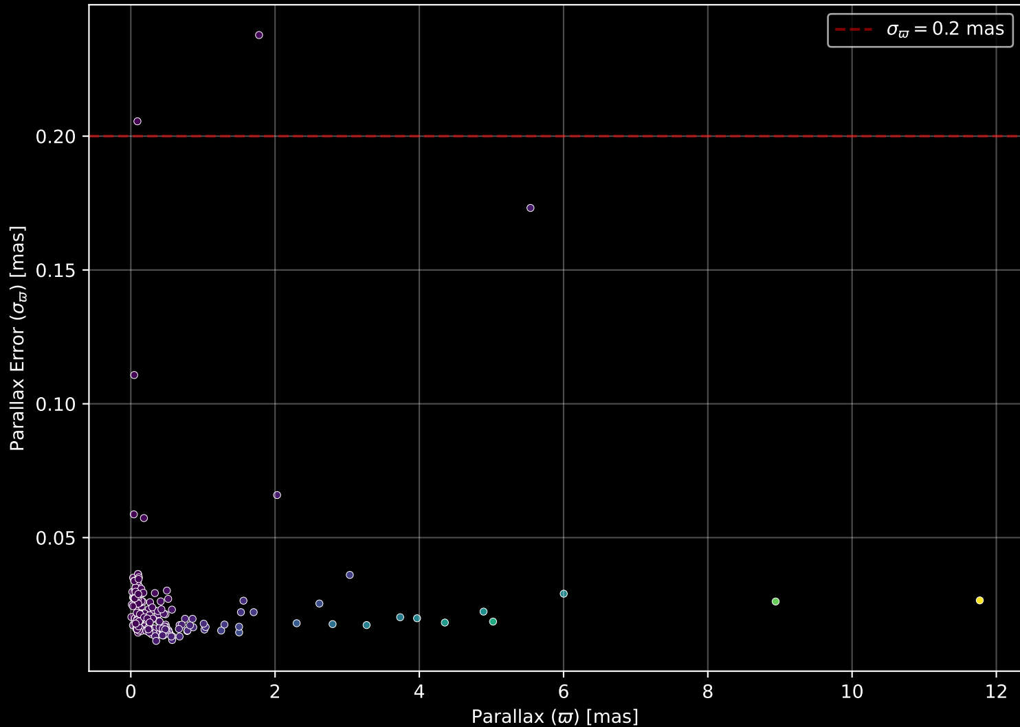
APOGEE DR17 Field: [M5] Parallax Quality (n= 185)
