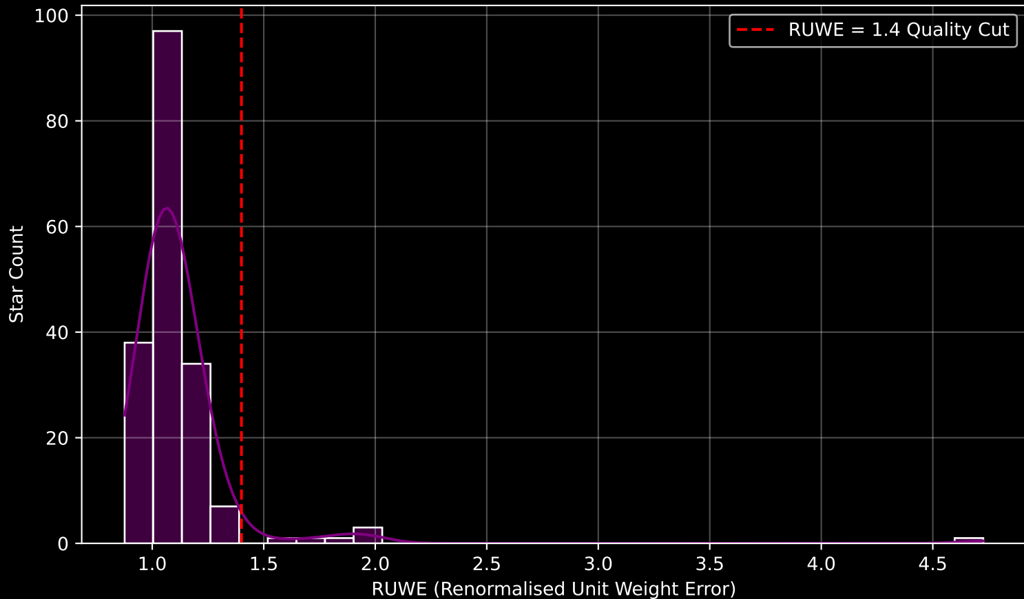
GAPOGEE DR17 Field [M5] RUWE Distribution (n= 183)
